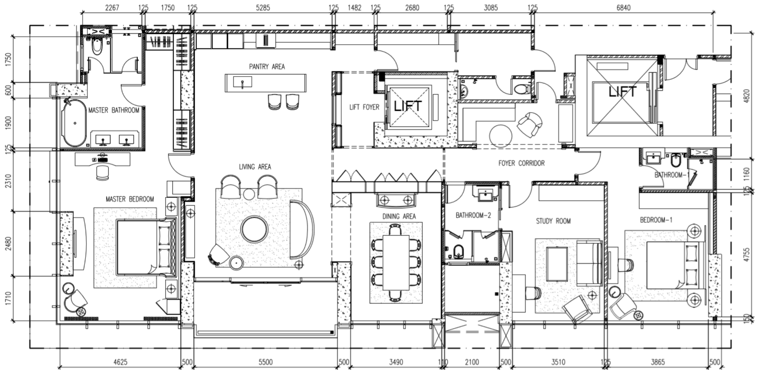
LAYOUT PLAN
