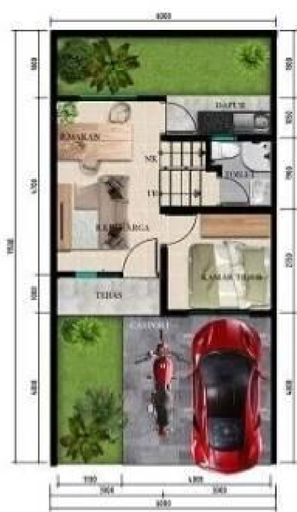
DENAH LT 1
